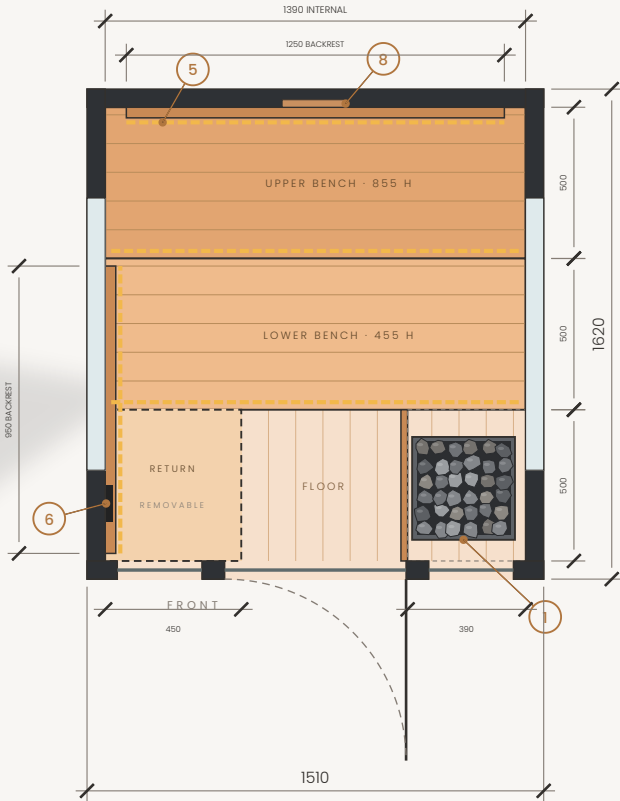
PLAN SCALE 1:25 · RETURN BENCH DASHED (OPTIONAL)
